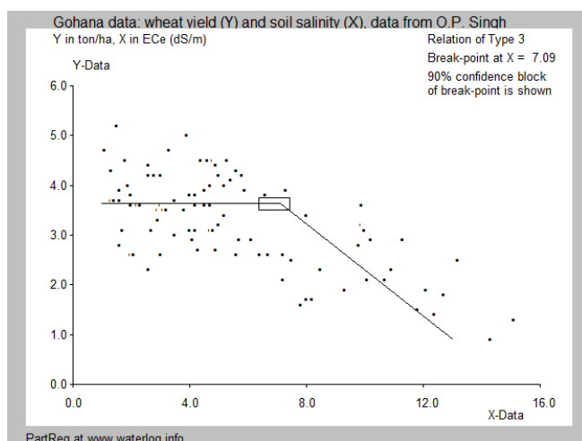
Fig. 3.3. Wheat at Gohana. BP=7 dS/m
