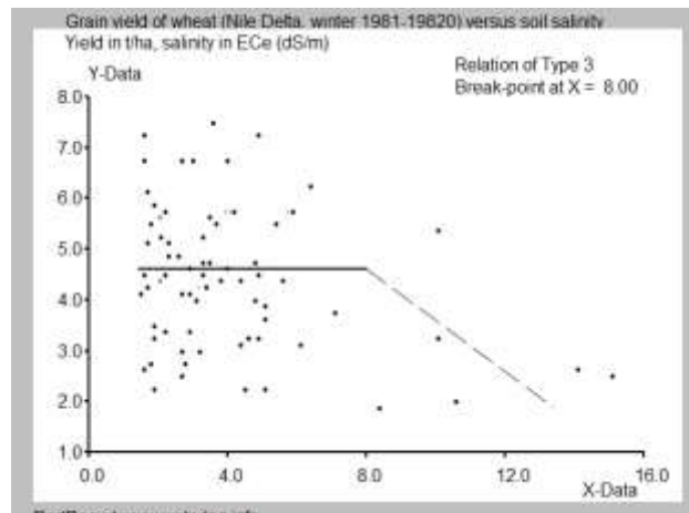
Fig. 1.5 Wheat. BP=8 dS/m
