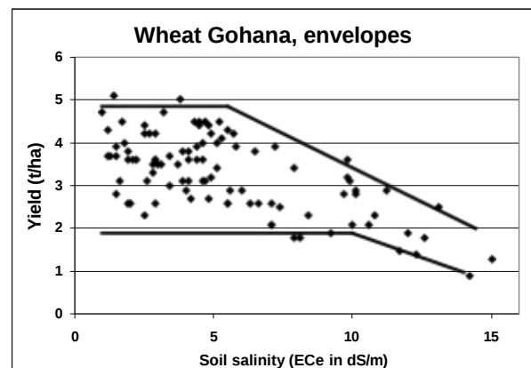
Fig. 5.1 Lower BP at ECe=6, upper BP at ECe=10
