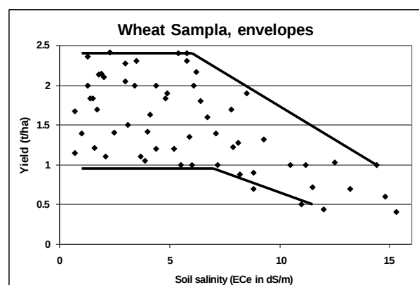
Fig 5.2 Lower BP at ECe=7, upper BP at ECe=8
